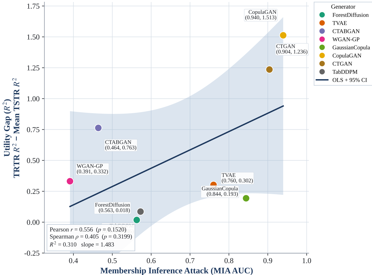
Concrete: MIA vs Utility Gap ( R^2 )
